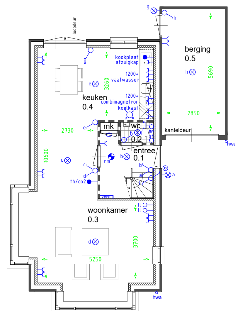
type A3 Begane grond
