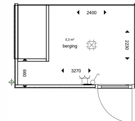
berging 1:50
