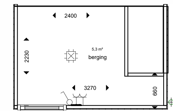
berging 1:50
