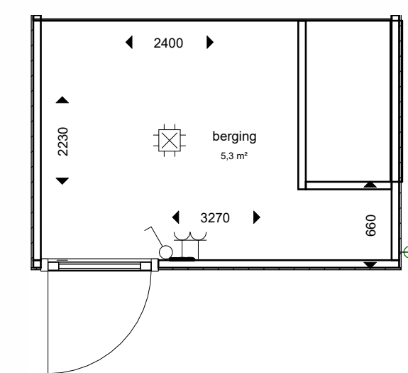
berging 1:50
