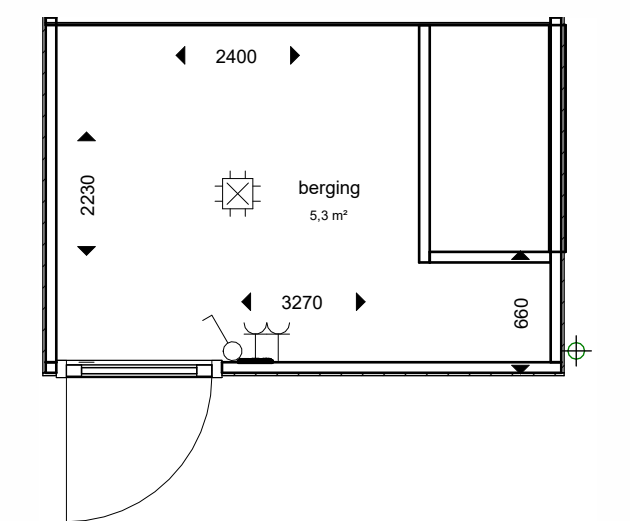
berging 1:50
