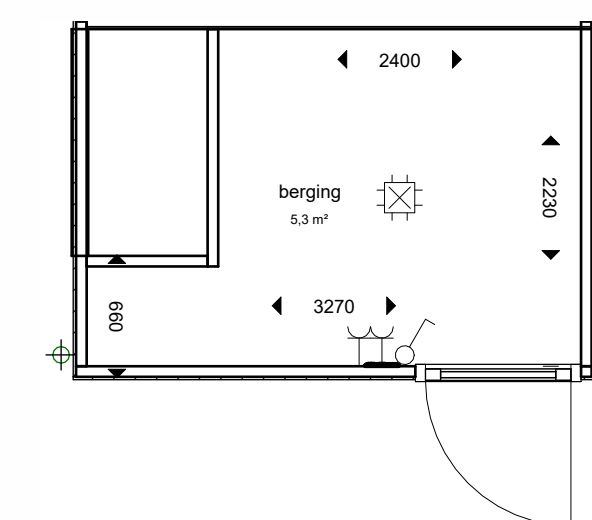
berging 1:50
