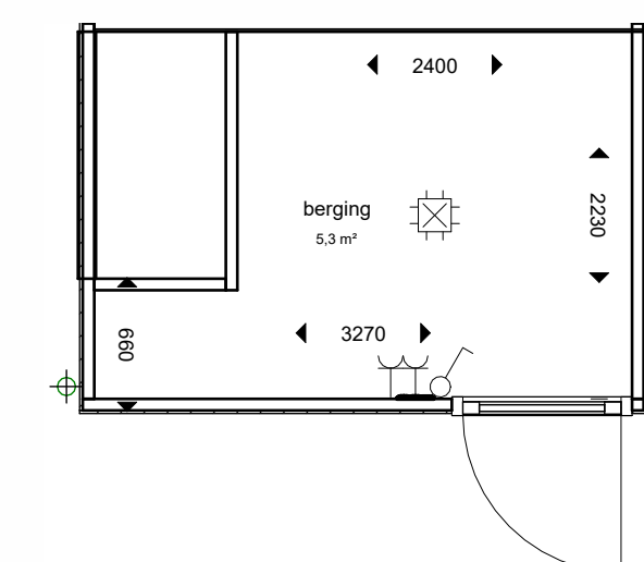
berging 1:50
