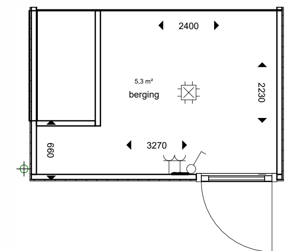
berging 1:50
