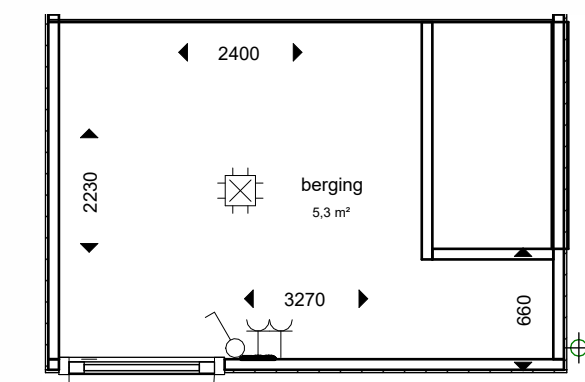
berging 1:50
