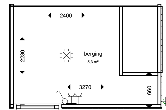
berging 1:50
