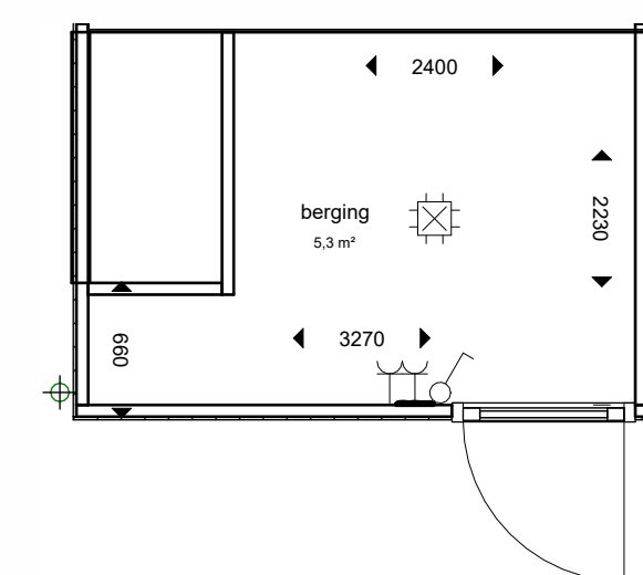
berging 1:50
