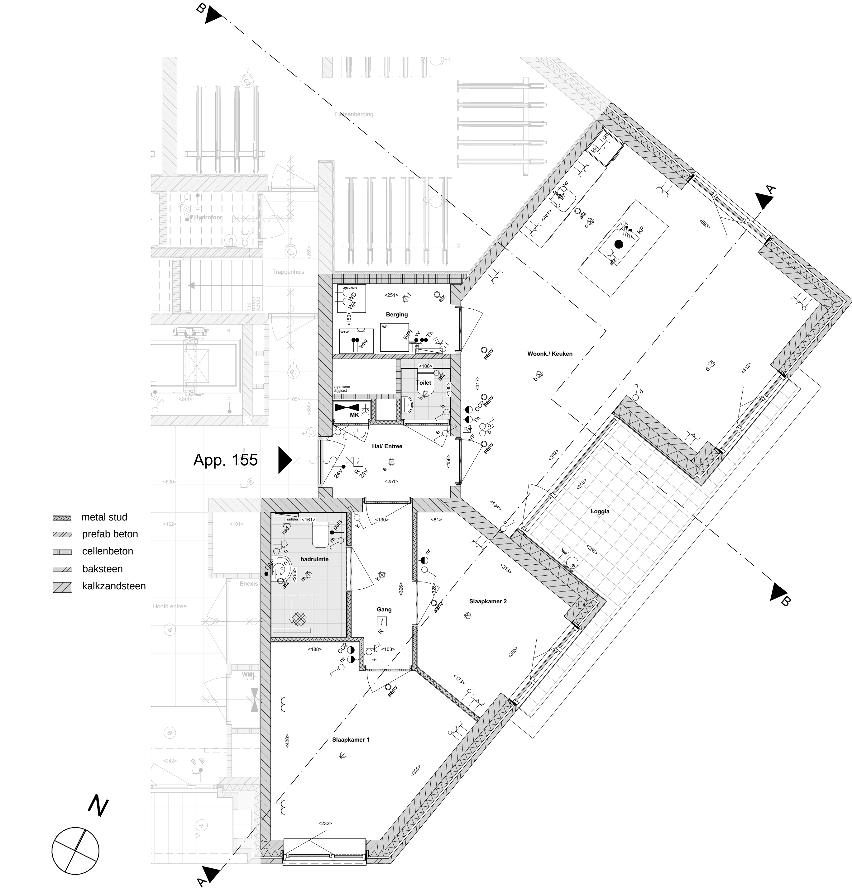
00 begane grond | 1:50
