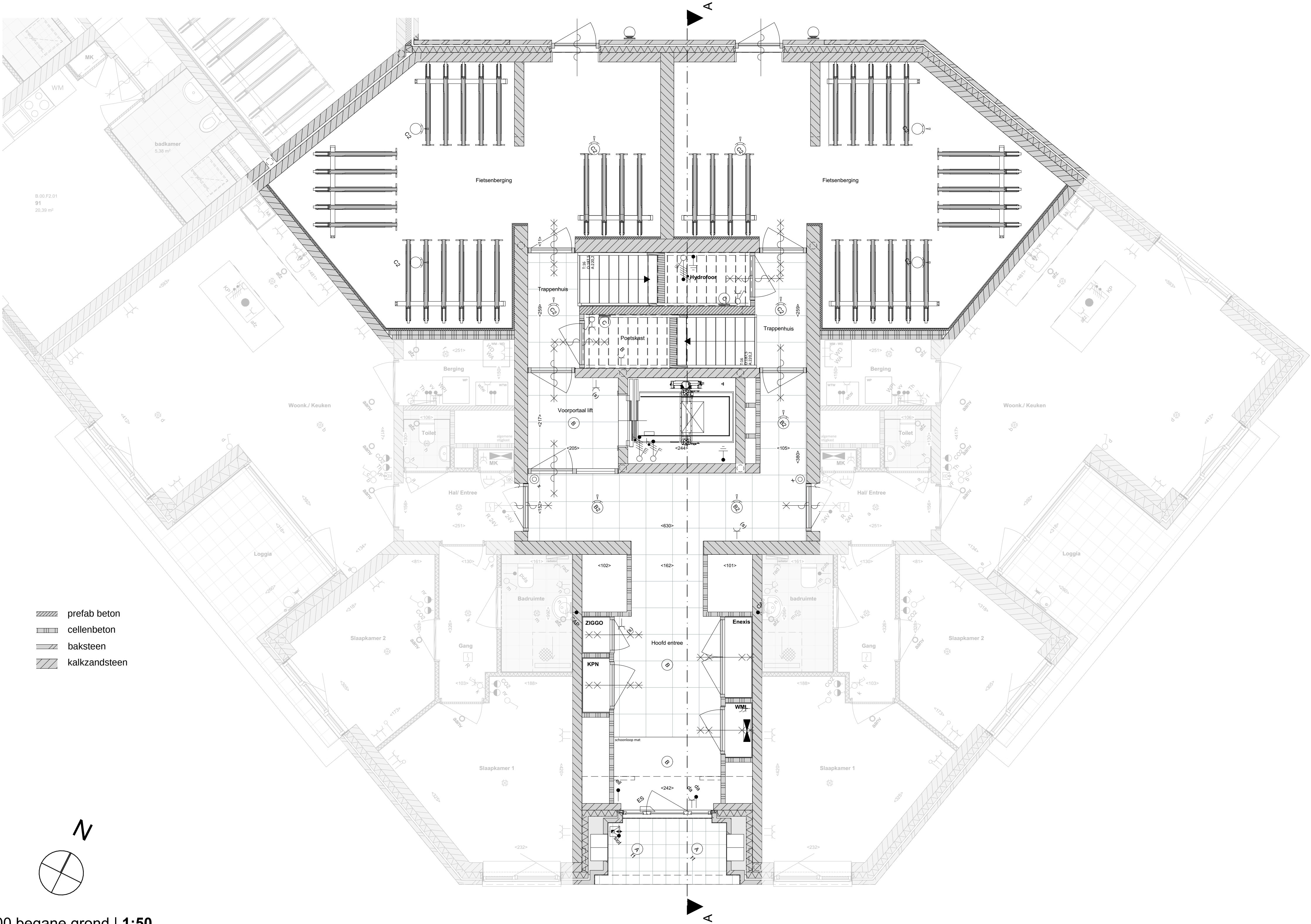
00 begane grond | 1:50
