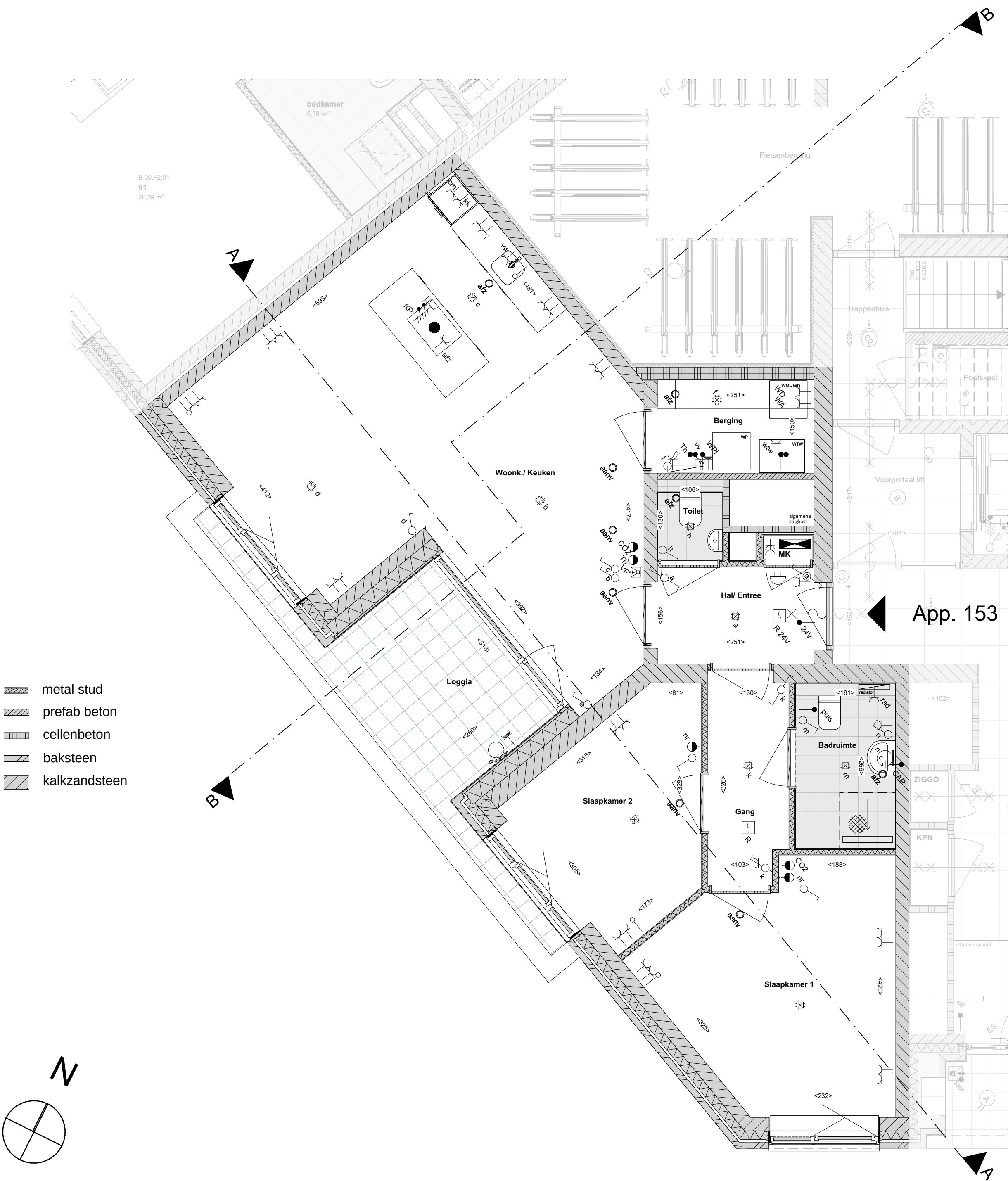
00 begane grond | 1:50
